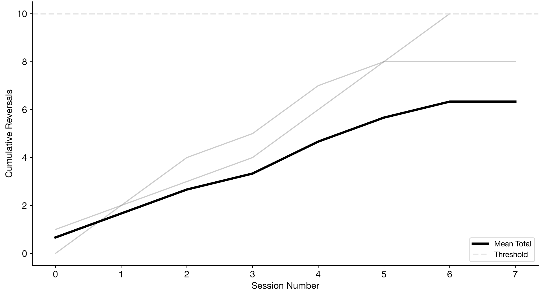
Cumulative Total Reversals Over Time (n=3 subjects; sessions per subject=1-8)
